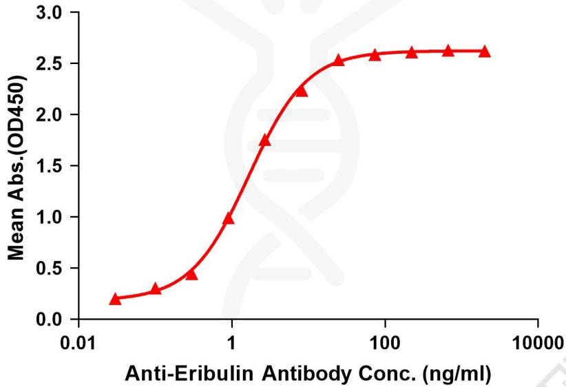
Figure 1. Elisa plates were pre-coated with IgG-Eribulin (0.2 \mu g/per well). Serial diluted anti-Eribulin monoclonal antibody (DME101049) solutions were added, washed, and incubated with secondary antibody before Elisa reading. From above data, the EC50 for anti-Eribulin monoclonal antibody binding with IgG-Eribulin is 1.670ng/ml.
