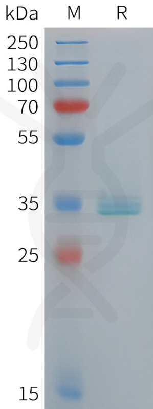
Figure 1. Human APOE Protein, His Tag on SDS-PAGE under reducing condition.
