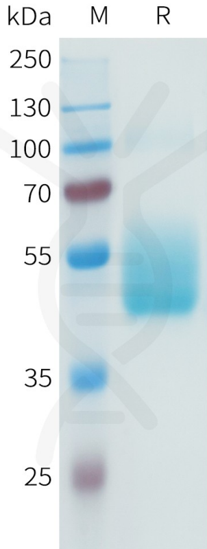
Figure 1. Human B7-H3(140-248) Protein, hFc Tag on SDS-PAGE under reducing condition.
