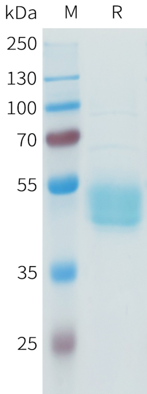
Figure 1. Human B7-H3(29-144) Protein, hFc Tag on SDS-PAGE under reducing condition.
