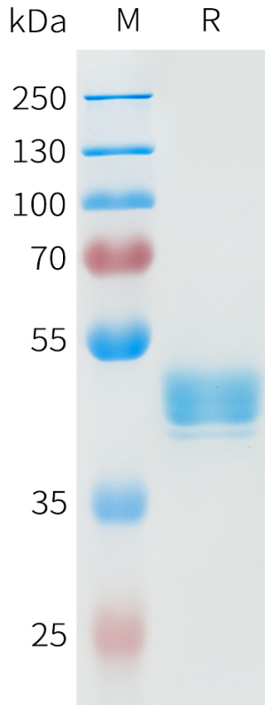
Figure 1. Human CDH3(108-215) Protein, hFc Tag on SDS-PAGE under reducing condition.
