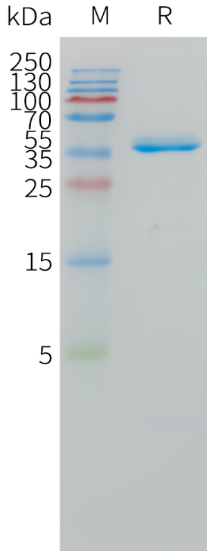
Figure 1. Human DLL3(428-492) Protein, hFc Tag on SDS-PAGE under reducing condition.
